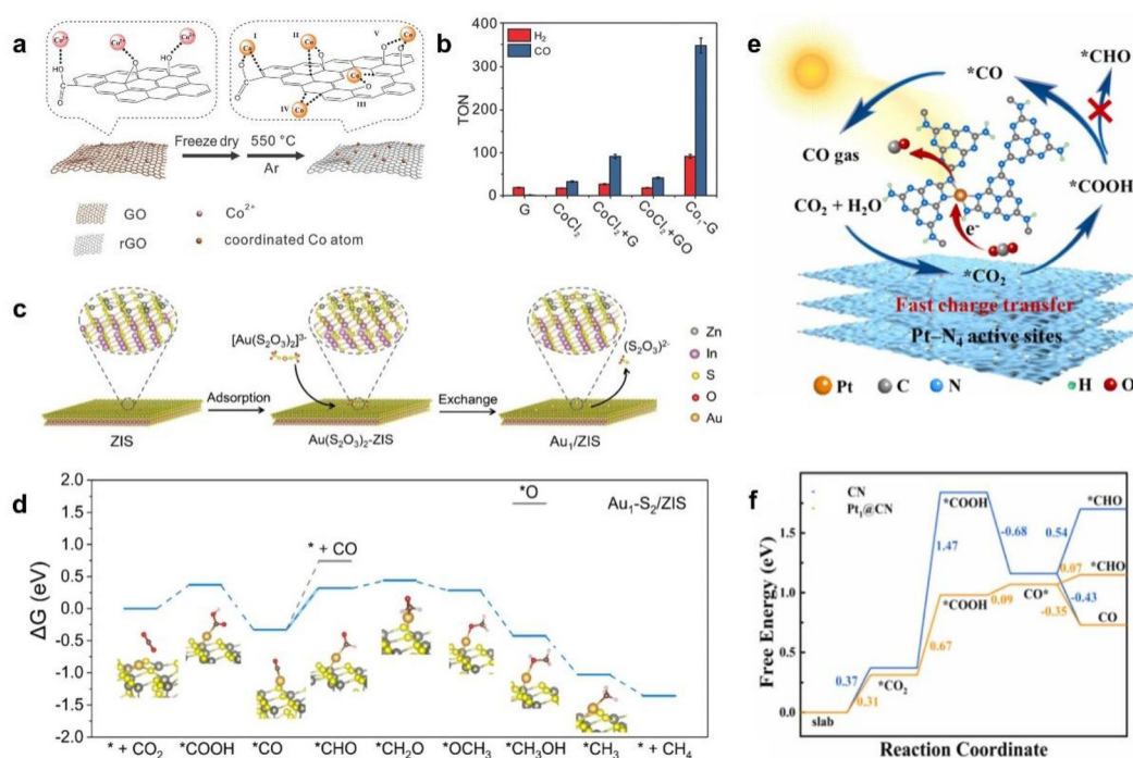
Fig. 9 (a) Diagrammatic overview of the Co1-G catalyst's synthesis, (b) TONs of \text{H}_2 and CO production across various catalysts. Reproduced with permission. 87 Copyright 2018, Wiley-VCH. (c) Schematic illustration for the preparation of \text{Au}_1/\text{ZIS} by a complex-exchange route, (d) free energy profile of \text{CO}_2 reduction on \text{Au}_1\text{-S}_2/\text{ZIS} catalysts. Reproduced with permission. 39 Copyright 2022, Wiley-VCH. (e) Mechanism of \text{CO}_2 reduction on Pt-N4 active sites under solar illumination, (f) free energy diagram for \text{CO}_2 reduction on CN and \text{Pt}_1@\text{CN} catalysts. Reproduced with permission. 50 Copyright 2024, Elsevier.
