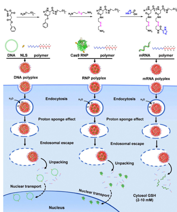
Fig. 9 Schematic depiction of the proposed intracellular pathways of the DNA polyplex, mRNA polyplex, and Cas9 RNP polyplex. In the cytosol, GSH cleaved the pendant –S–S– bonds in the polymers, thereby converting the cationic polymers to neutral polymers and thus releasing the payloads. Adapted with permission from ref. 121, Copyright 2018, American Chemical Society.
