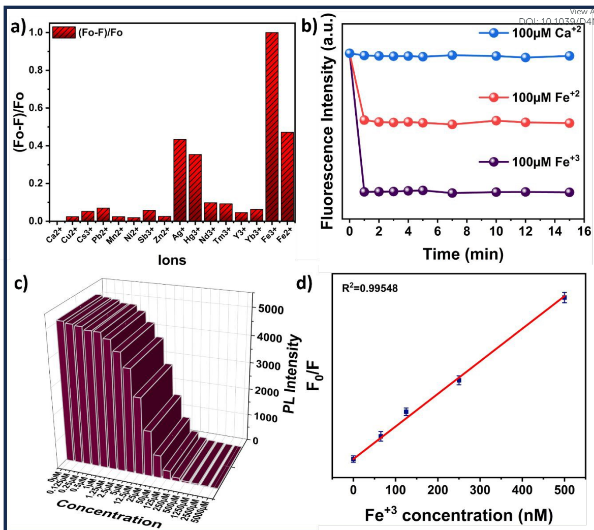
Figure 5: (a) Bar graph illustrating the fluorescence-based selectivity response of MQDs over a series of different heavy metal ions, (b) the response time optimization of the MQDs after the addition of Fe^{3+} ions, (c) Fe^{3+} concentration-dependent fluorescence quenching study of MQDs, (d) linear function describing fluorescence quenching by Fe^{3+} ions (concentration range 0 nM to 500 nM).
