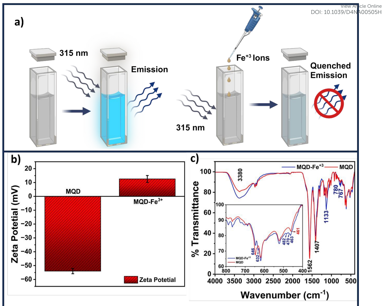
Figure 7: (a) Schematic representing the mechanism of fluorescence quenching of MQDs in the presence of Fe 3+ ions, (b) zeta potential measurements of MQDs and MQD with Fe 3+ ions in ultrapure water, (c) FTIR spectrum of MQDs and MQD with Fe 3+ ions.
