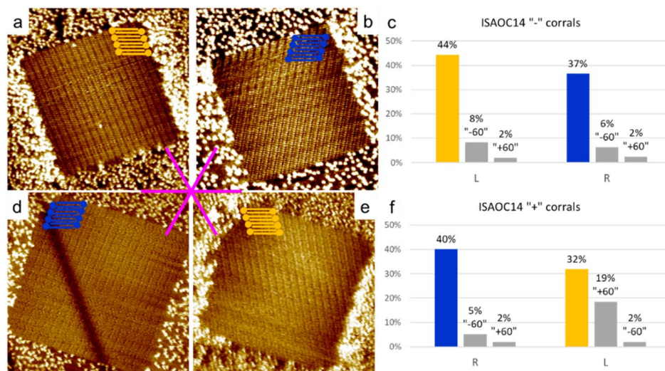
Fig. 5 STM images of “-” corrals (60 × 60 nm) containing the main (a) and the second most frequent (b) self-assembled structure formed by ISA-OC14 (imaging parameters: V_{\text{bias}}: -0.700 V, I_{\text{set}}: 0.070 nA). Schematic models of the self-assembled structure are shown in the corner of the corrals. Graph showing the percentage distribution of self-assembled structure in “-” corrals filled with ISA-OC14 (c). All three “L” rotational domains are grouped together in the first cluster of bars, while the three “R” rotational domains are grouped together in the second cluster of bars. STM images of “+” corrals (60 × 60 nm) containing the main (d) and the second most frequent (e) self-assembled structure formed by ISA-OC14 (imaging parameters: V_{\text{bias}}: -0.700 V, I_{\text{set}}: 0.070 nA). Schematic models of the self-assembled structure are shown in a corner of the corrals. Graph showing the percentage distribution of self-assembled structure in “+” corrals filled with ISA-OC14 (f). All three “R” rotational domains are grouped together in the first cluster of bars, while the three “L” rotational domains are grouped together in the second cluster of bars. For the grey bars relative to the rotational domains in (c and f), an indication of which specific domain is reported as a “+60” or as a “-60”. These values indicate the angle of rotation compared to the corresponding main domain. The statistics are based on 302 corrals (205 for “-” corrals, 97 for “+” corrals). The concentration of ISA-OC14 is 5.3 \times 10^{-4} M. The unit cell vector a of the main domain is not always perfectly parallel to the lateral side of the corral (as discussed in the main text).
