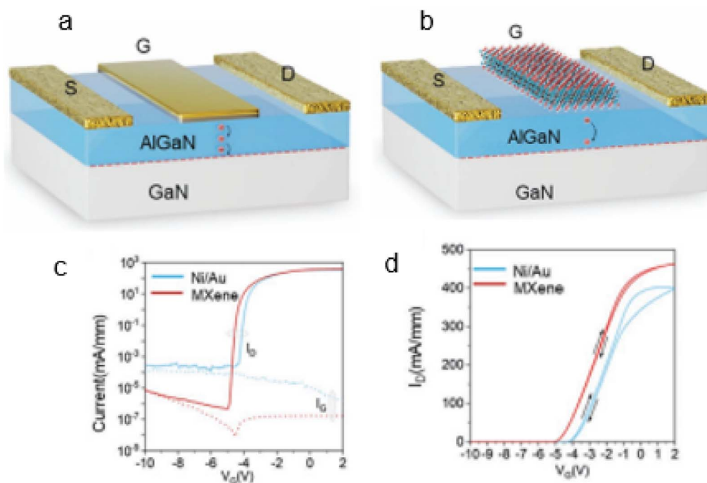
Fig. 18 GaN HEMT schematic diagrams with either Ti 3 C 2 T x or (a) Ni/Au or (b) the gate electrodes. (c) The Ni/Au- and MXene-gate GaN HEMTs' I_D curves and logarithmic-scale transfer curves. (d) GaN HEMT dual-sweep transfer curves on a linear scale (copyright 2023 John Wiley and Sons).
