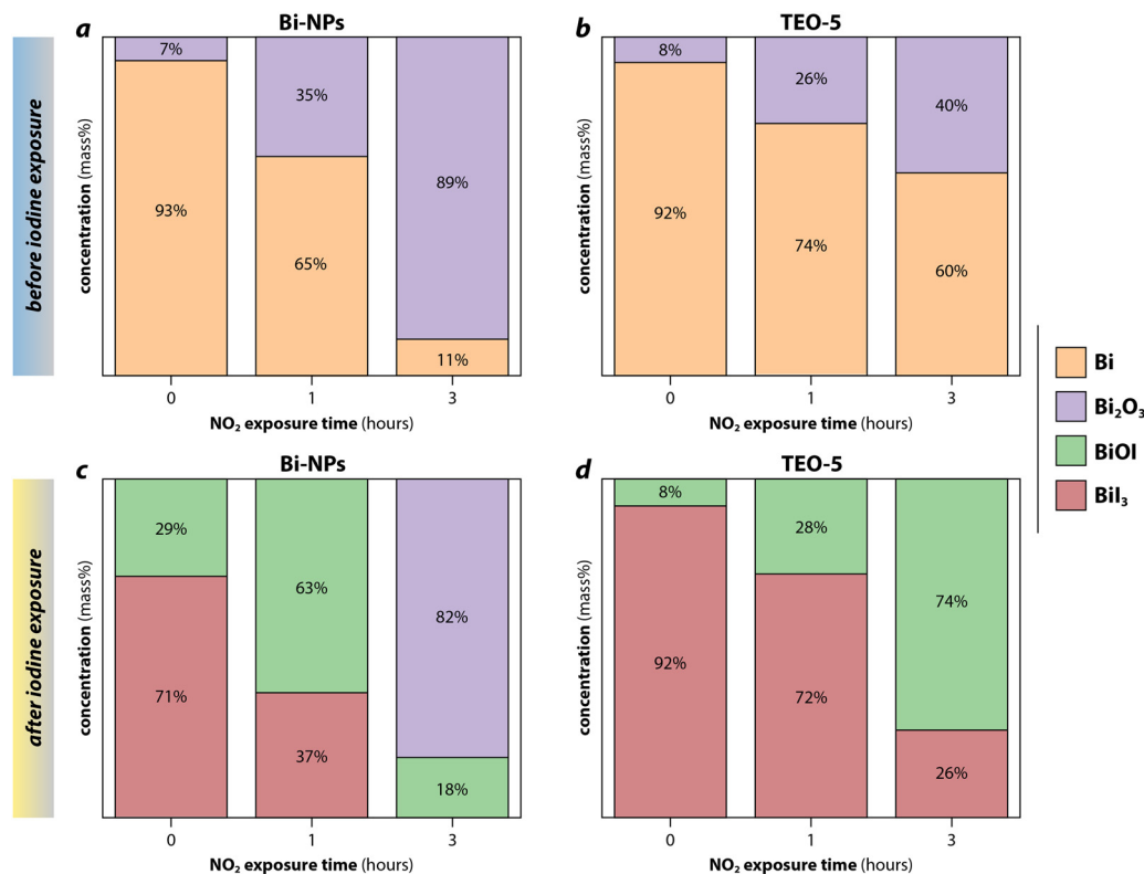
Fig. 8 Results from Rietveld refinement applied on X-ray diffraction data of (a) bismuth nanoparticles (Bi-NPs) and (b) silica xerogels (TEO-5) loaded with Bi-NPs after 0 h, 1 h, and 3 h of 1 v/v% \text{NO}_2 aging, and the same samples after subsequent iodine exposure (c) Bi-NPs and (d) TEO-5. The bismuth-compounds formed after aged samples were exposed to iodine is dependent upon the Bi:Bi 2 O 3 ratio. When Bi 2 O 3 was greater than 50% after aging, as for 3 h shown in (a), only BiOI and Bi 2 O 3 were present after iodine exposure, as shown in (c). For aged samples with less than 50% Bi 2 O 3 , BiI 3 , and BiOI were present as shown in (c) 0-h and 1-h aged Bi-NPs and (d) 0–3 h aged TEO-5. This figure was recreated from Baskaran et al. 105 and reprinted with permission. Copyright 2022 Elsevier.
