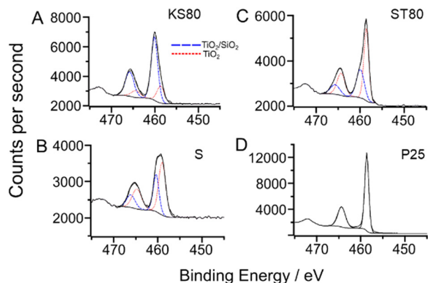
Fig. 5 Fitted high resolution Ti 2p X-ray photoelectron scans of: A-sample KS80, B-sample S, C-sample ST80 and D-P25 TiO 2 standard. Fitted environments for KS80, S and ST80 were the same as those in our previous paper, 29 with a doublet separation of 5.72 eV. Samples KS80, S and ST80 exhibited differing ratios of TiO 2 to TiO 2 /SiO 2 components, as listed in Table 2.
