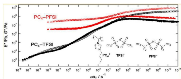
Fig. 27 Elastic modulus of imidazolium-based polymerized ionic liquids upon introducing large counteranions. Reproduced from ref. 43 with permission from ACS, Copyright [2018].
