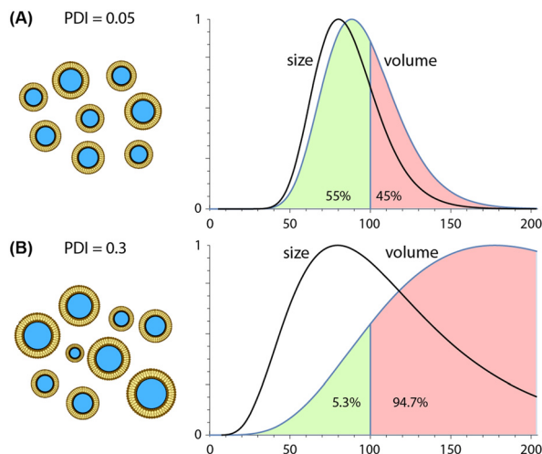
Fig. 4 Impact of nanoparticle polydispersity on drug delivery. Comparison of nanoparticle populations with identical modal diameters of 80 nm but different size distributions. Each distribution is defined by a probability density function (PDF) reflecting a PDI value of either (A) 0.05 or (B) 0.3. For each case, both size (diameter) and volume distributions (PDF scaled by the size-dependent particle volume) are presented. Plots are normalized by modal peak values.
