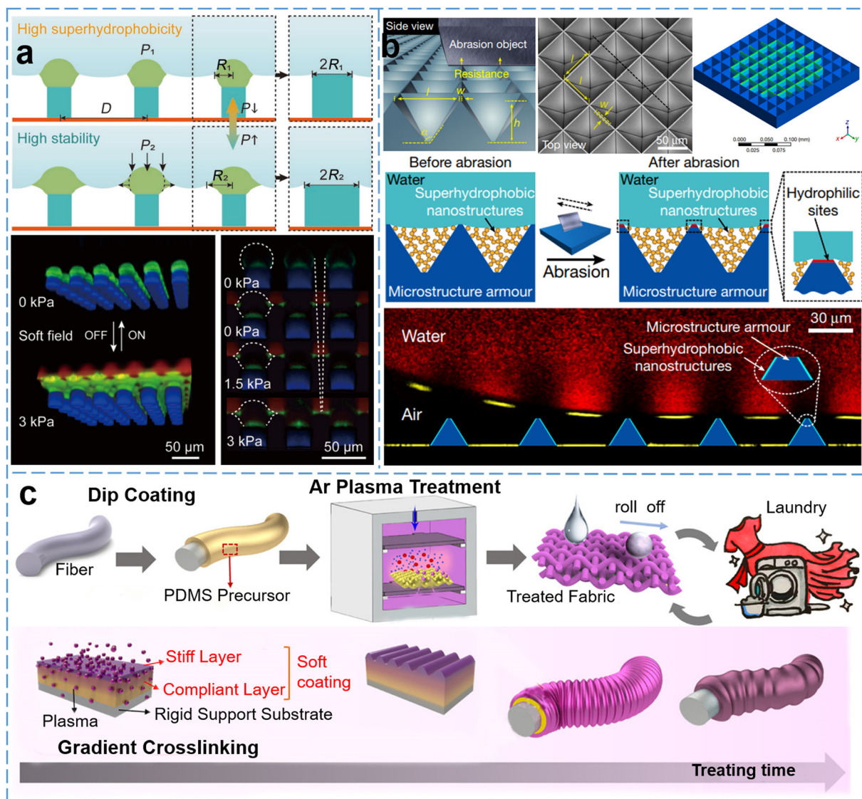
Fig. 7 (a) Design of the LPGSS and its switching effect diagram, 132 Copyright 2022 Wiley-VCH; (b) design of the microstructure armour, 133 Copyright 2020 Springer Nature; (c) SH fabric is prepared by argon plasma treatment and a wrinkled surface is formed on the fiber, 134 Copyright 2021 American Chemical Society.
