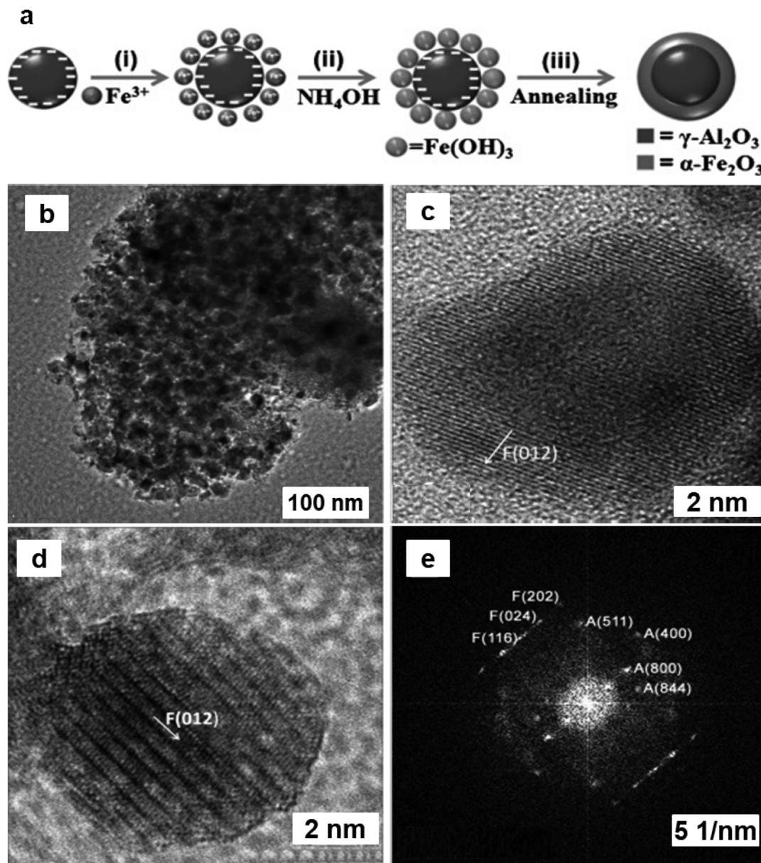
Fig. 32 (a) Schematic synthesis of \text{Al}_2\text{O}_3@ \text{Fe}_2\text{O}_3 mesoporous core-shell catalyst; (b–d) TEM images of \text{Al}_2\text{O}_3@ \text{Fe}_2\text{O}_3 -2; (e) Crystal structures of \gamma\text{-Al}_2\text{O}_3 (A) and \alpha\text{-Fe}_2\text{O}_3 (F). Reproduced with permission from ref. 219 Copyright 2013, Wiley-VCH GmbH & Co. KGaA, Weinheim.
