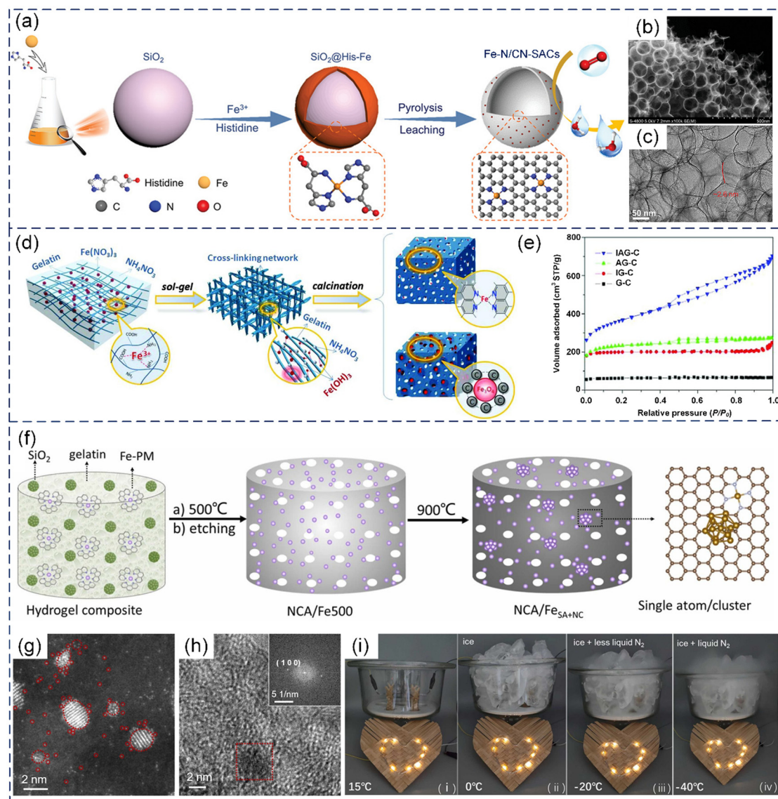
Fig. 13 (a) Schematic illustration of the synthetic process, (b) SEM image, and (c) TEM image of Fe-N/CN-SACs. (a)–(c) Reproduced with permission from ref. 63 (Copyright 2018, Wiley). (d) Illustration of the procedure for the preparation of IAG-C catalysts ( i.e. , Fe-N-C catalyst: \text{Fe}(\text{NO}_3)_3 , \text{NH}_4\text{NO}_3 , and gelatin as precursor components) and \text{Fe}_3\text{O}_4@\text{AGC} ( \text{Fe}_3\text{O}_4/\text{N} -doped carbon hybrid) electrode materials. (e) Nitrogen adsorption–desorption curves of four samples prepared with different precursors (AG-C: ammonium nitrate and gelatin; IG-C: iron nitrate and gelatin; and G-C: pure gelatin). (d) and (e) Reproduced with permission from ref. 207 (Copyright 2015, AAAS). (f) Schematic illustration of the preparation of NCA/ \text{Fe}_{\text{SA}+\text{NC}} . (g) HAADF-STEM images of NCA/ \text{Fe}_{\text{SA}+\text{NC}} . (h) High-resolution transmission electron microscopy (HRTEM) image of a typical metal cluster in NCA/ \text{Fe}_{\text{SA}+\text{NC}} . The inset shows the Fourier transform of the red region. (i) Photographs of an LED pattern powered by two Zn//NCA/ \text{Fe}_{\text{SA}+\text{NC}} batteries in series at different temperatures. (f)–(i) Reproduced with permission from ref. 210 (Copyright 2023, ScienceDirect).
