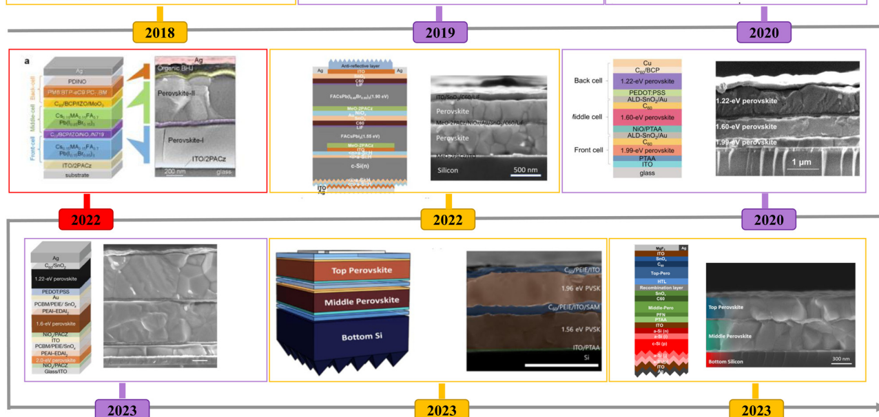
Fig. 6 Structure evolution and cross sectional SEM images of perovskite-based triple-junction solar cells. Reproduced with permission from ref. 14–17, 22–26. Copyright © 2018, American Chemical Society. Copyright © 2019 Published by Elsevier Inc. Copyright © 2020, Wang et al. , Published by Springer Nature, Copyright © 2020, American Chemical Society, Copyright © 2022, American Chemical Society, Copyright © 2022, American Chemical Society, Copyright © 2023, Wang et al. under exclusive licence to Springer Nature Limited, Copyright © 2023, American Chemical Society, Copyright © 2023 Heydari et al. , Published by American Chemical Society.
