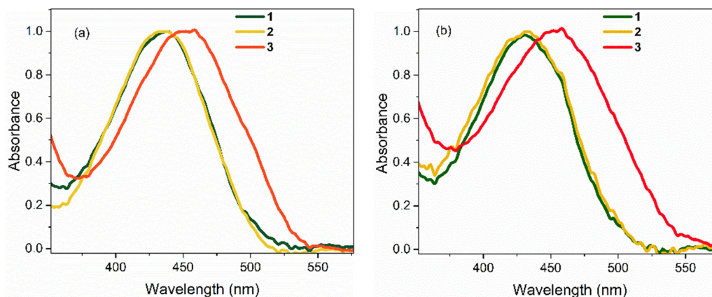
Fig. 2 Steady-state absorption spectra of 1–3 at T = 298 K in: (a) EtOH, and (b) THF. In both solvents, the spectra for 1 and 2 are nearly identical. All spectra are normalised to unit intensity.
