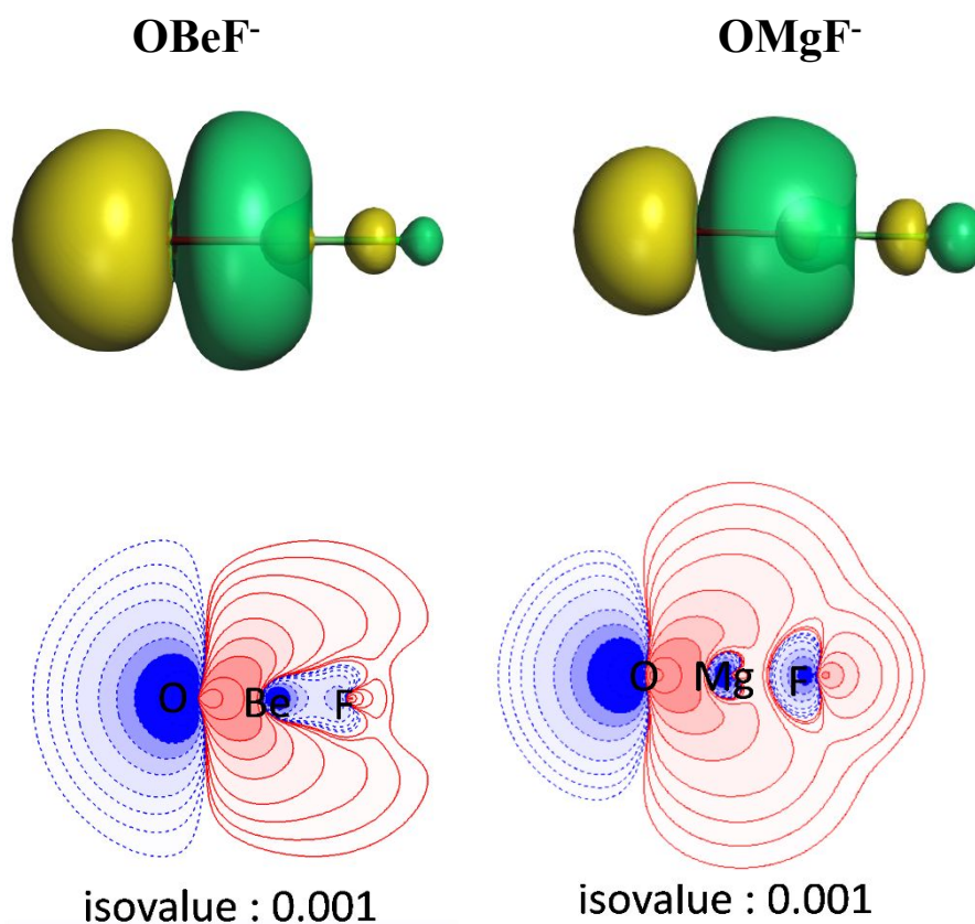
Fig.5: (Top): Plot of the 3D shape of the HOMO-1 orbitals with an isovalue of 0.03 \text{ e/au}^3 of OBeF - and OMgF - and (bottom) contour line plot of the same orbital HOMO-1 in the plane containing the bond axis with different isovalues at the BP86/def2-TZVPP level. The isovalue below each plot represents the value of the outermost contour in the graph, and the values for the contour settings are in the order of 0.001, 0.002, 0.004, 0.008, 0.02, 0.04, 0.08, 2.0, 4.0 \text{e/au}^3 .
