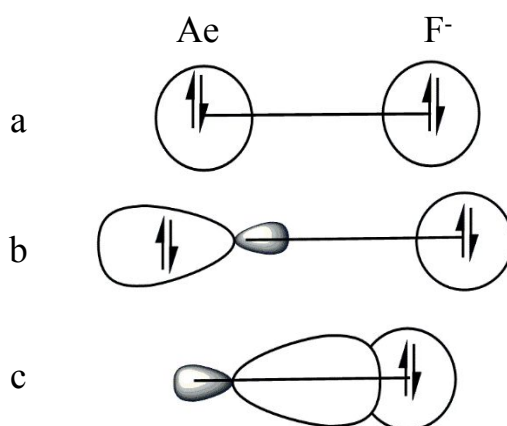
Fig.12: Schematic representation of the \sigma bond formation in \text{AeF}^- in three steps. (a) Initial charge distribution in \text{Ae} atom and \text{F}^- where the arrows indicate the total electronic charge; (b) Polarization of the valence electrons in \text{Ae} and (n)s^2 \rightarrow (n)s/p(\sigma) hybridization; (c) Concomitant formation of the vacant orthogonal (n)s/p(\sigma) orbital at \text{Ae} atom which overlaps with the occupied \sigma orbitals of \text{F}^- which leads to a polar covalent \text{Ae-F}^- bond.
