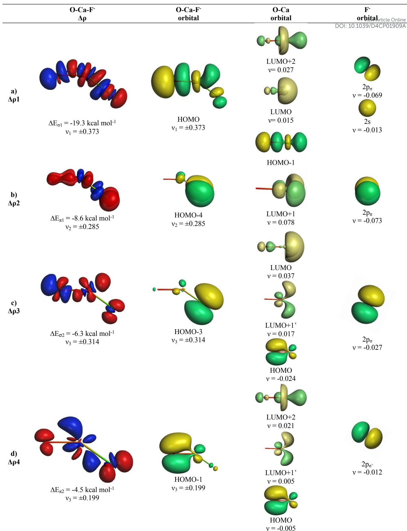
Fig.7: Plot of deformation densities \Delta\rho of \text{OCaF}^- . The pairwise orbital interactions and the associated interaction energies ( \Delta E_{\text{orb}} ) between fragments \text{OCa(S)} and \text{F}^-(\text{S}) in \text{OCaF}^- at the equilibrium structure, as well as the shape of the most important interacting MOs. The direction of the charge flow is red→blue. (Isovalue 0.03e/\text{au}^3 ).
