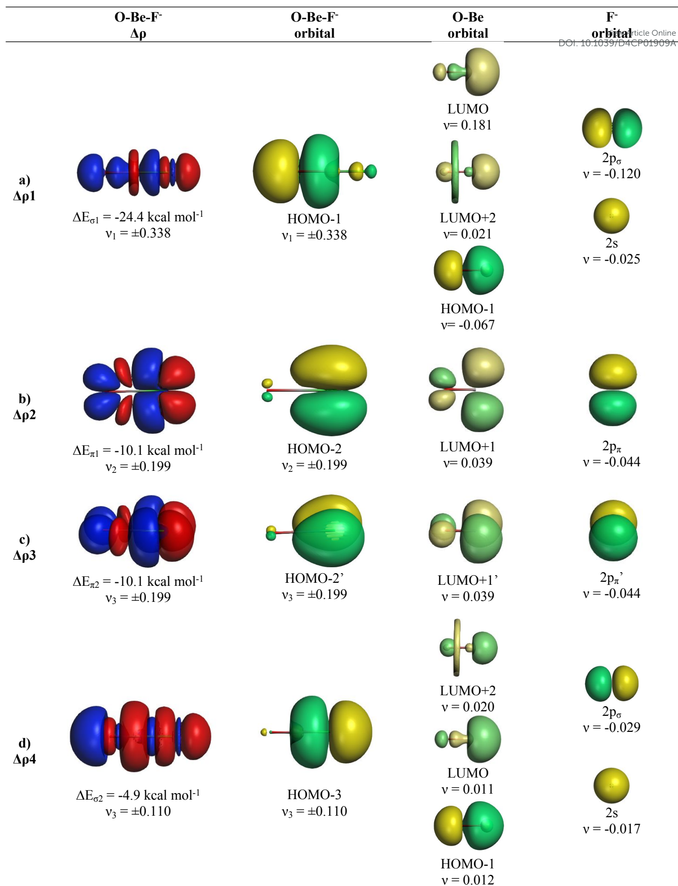
Fig.4: Plot of deformation densities \Delta\rho of OBeF - . The pairwise orbital interactions and the associated interaction energies ( \Delta E_{\text{orb}} ) between fragments OBe(S) and F - (S) in OBeF - at the equilibrium structure as well as the shape of the most important interacting MOs. The direction of the charge flow is red→blue. (Isovalue 0.03e/au 3 ).
