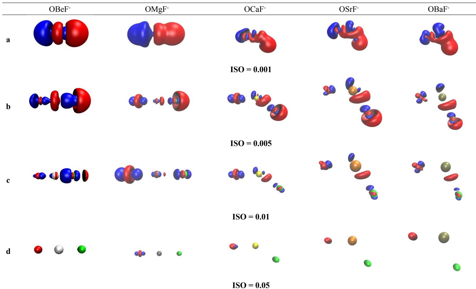
Fig.3: Charge density difference maps at the BP86/def2-QZVPP level. \text{OAEF}^- and the fragments \text{OAE} + \text{F}^- ( \text{Ae} = \text{Be, Mg, Sr} ) with different values for the isodensity surfaces \text{Iso} given in \text{e}/\text{au}^3 . The direction of the charge flow is red→blue.
