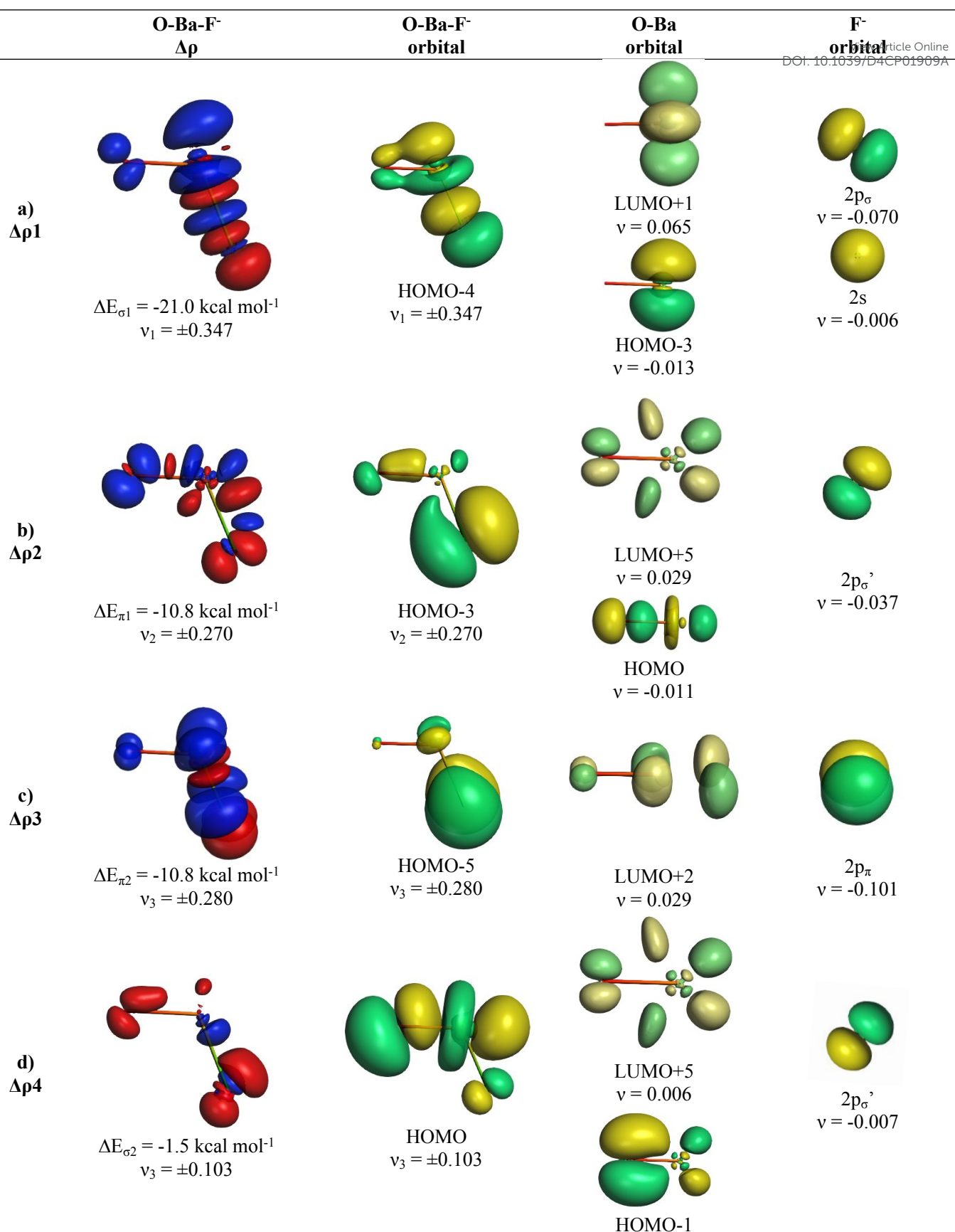
Figure 9. Plot of deformation densities \Delta\rho of \text{O}^+\text{BaF}^- . The pairwise orbital interactions and the associated interaction energies ( \Delta E_{\text{orb}} ) between fragments \text{O}^+\text{Ba}(\text{S}) and \text{F}^-(\text{S}) in \text{O}^+\text{BaF}^- of the bent equilibrium structure, as well as the shape of the most important interacting MOs. The direction of the charge flow is red→blue. (Isovalue 0.03e/\text{au}^3 ).
