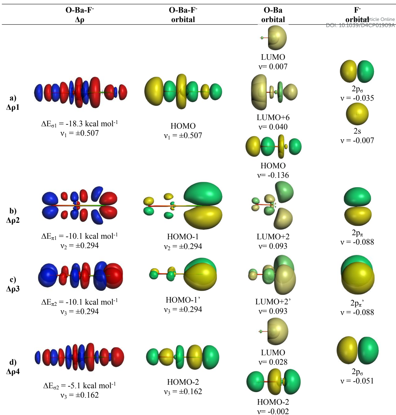
Fig.10: Plot of deformation densities \Delta\rho of OBaF - . The pairwise orbital interactions and the associated interaction energies ( \Delta E_{\text{orb}} ) between fragments OBa(S) and F - (S) in OBaF - of the linear structure, as well as the shape of the most important interacting MOs. The direction of the charge flow is red→blue. (Isovalue 0.03e/\text{au}^3 ).
