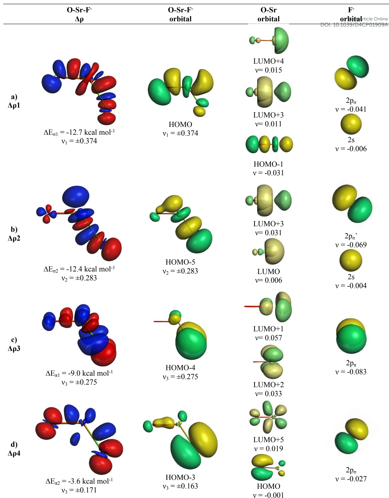
Fig.8: Plot of deformation densities \Delta\rho of OSrF - . The pairwise orbital interactions and the associated interaction energies ( \Delta E_{\text{orb}} ) between fragments OSr(S) and F(S) in OSrF - at the equilibrium structure, as well as the shape of the most important interacting MOs. The direction of the charge flow is red→blue. (Isovalue 0.03e/\text{au}^3 ).
