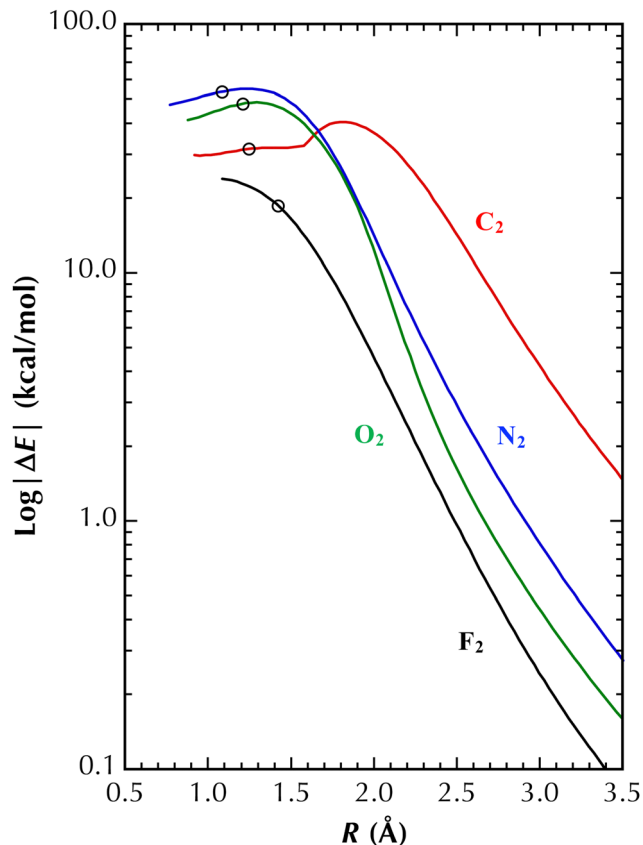
Fig. 5 Variation of \log|\Delta E_{\text{DEC}}(R)| for the A_2 molecules. The circles are located at the calculated equilibrium internuclear distances, R_e , for each molecule.
