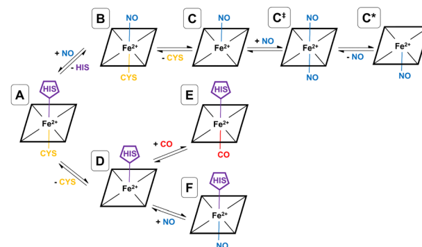
Fig. 2 Gaseous inhibitory pathways shown in hCBS. Species A , B , C , D , and E have been experimentally observed, and C and E are the final inhibitory states for NO and CO, respectively. Species C ‡ , C * and F are not experimentally observed, but are computationally and biochemically suggested in this work.
