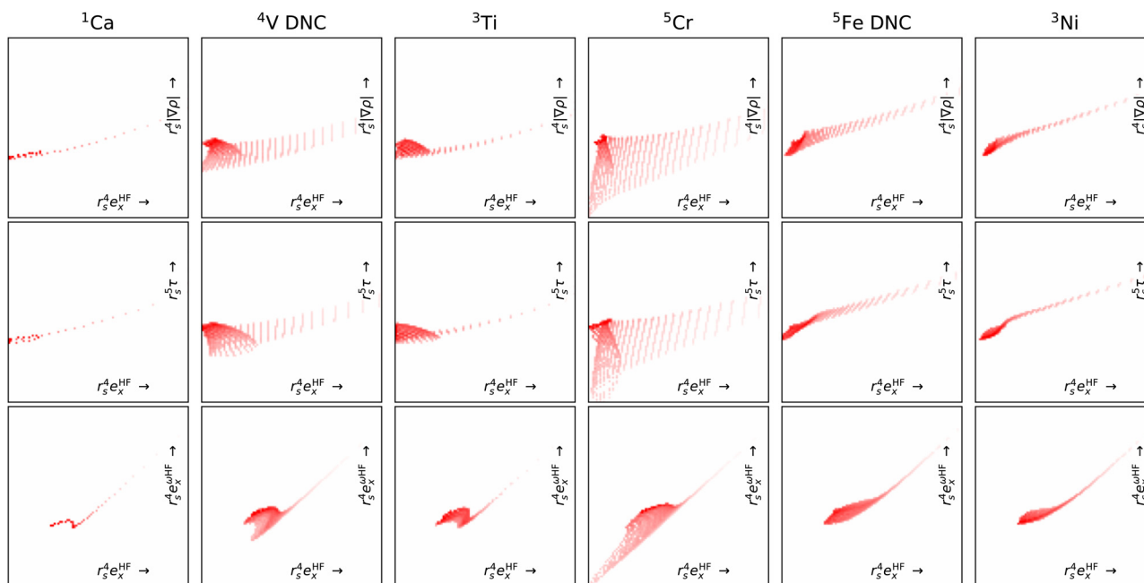
Fig. 8 Like Fig. 7 but for atoms (columns) and with fewer features pairs (rows). Note, of these atoms V and Fe did not converge (DNC) using any strategy.
