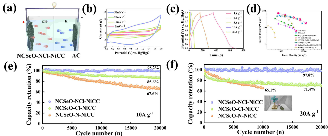
Fig. 6 (a) Structure schematic of the NCSeO–NCl–NiCC//AC ASC device. (b) CV curves of the ASC device of NCSeO–NCl–NiCC//AC at different scan rates. (c) GCD curves of the ASC device of NCSeO–NCl–NiCC//AC at different current densities. (d) Ragone plots of NCSeO–NCl–NiCC//AC compared with different electrical energy-storage technologies. Cycling stability of the NCSeO–NCl–NiCC//AC ASC device at (e) 10 A g -1 and (f) 20 A g -1 .
