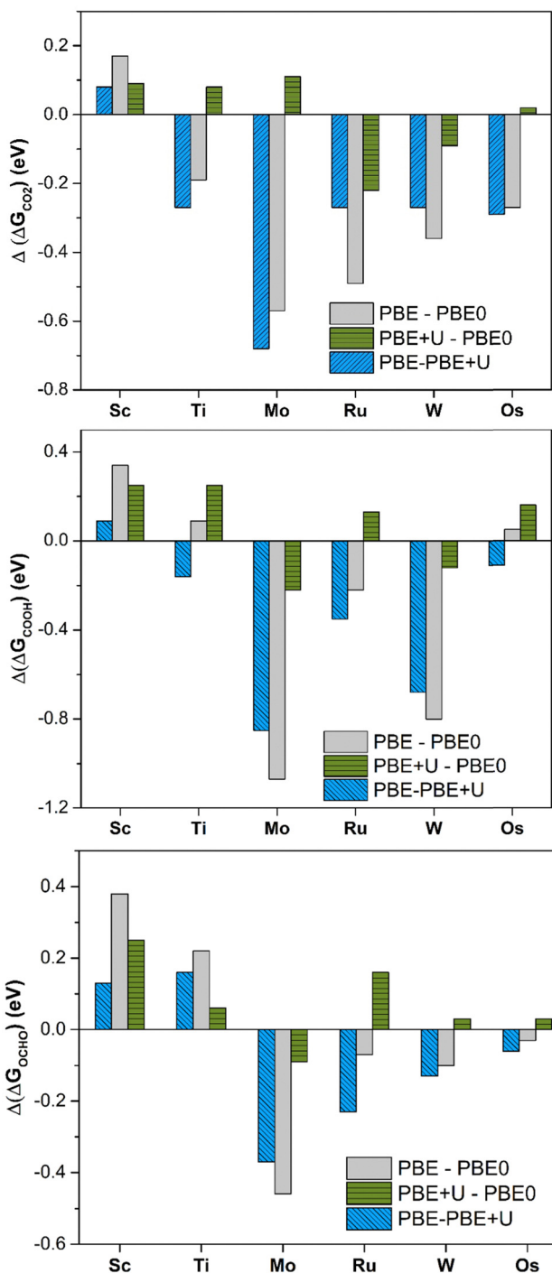
Fig. 2 Deviation of Gibbs free energies comparing different levels of theory for *CO 2 , *COOH, and *OCHO adsorption on TM@4N-Gr.
