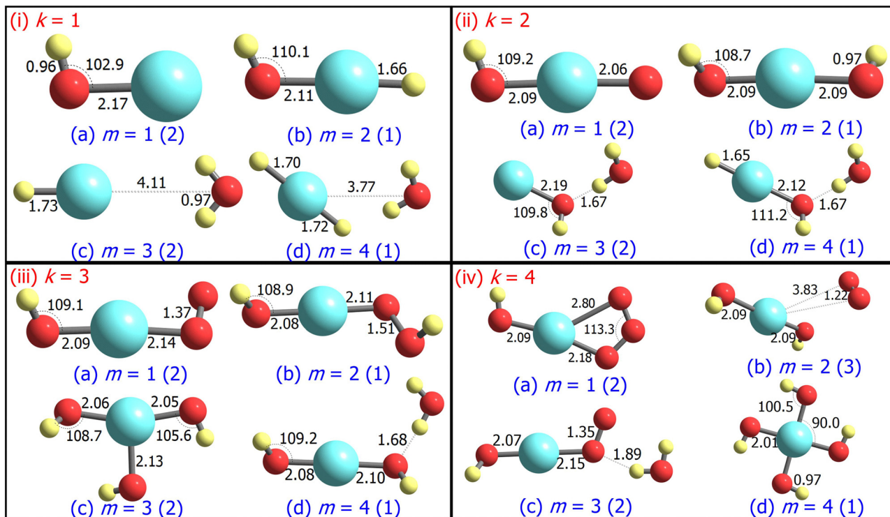
Fig. 2 Ground state structures of \text{AgO}_k\text{H}_m^- , where k, m = 1-4 , optimized at the CCSD level. Bond lengths and angles are given in Ångströms and degrees, respectively. The spin multiplicity ( 2S + 1 ) of the \text{AgO}_k\text{H}_m^- clusters is provided in the parentheses.
