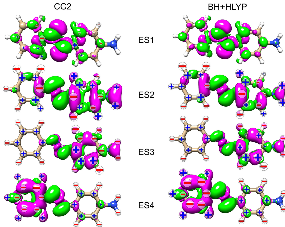
Fig. 9 AZO-2. RI-CC2 and TD-DFT/BH+HLYP (aug-cc-pwCVVDZ basis set) difference densities for the four lowest excited states (ES) with the sign (+/−) of the nuclei's \mathcal{L}_K \mathcal{B}_K terms. The size of the sign indicates the magnitude (magnified by 1000) of the signal (smallest for 1 < |\text{NSCD}| < 10 , middle size for 10 < |\text{NSCD}| < 100 and largest for |\text{NSCD}| > 100 . NSCD signals with absolute values < 1 are not shown).
