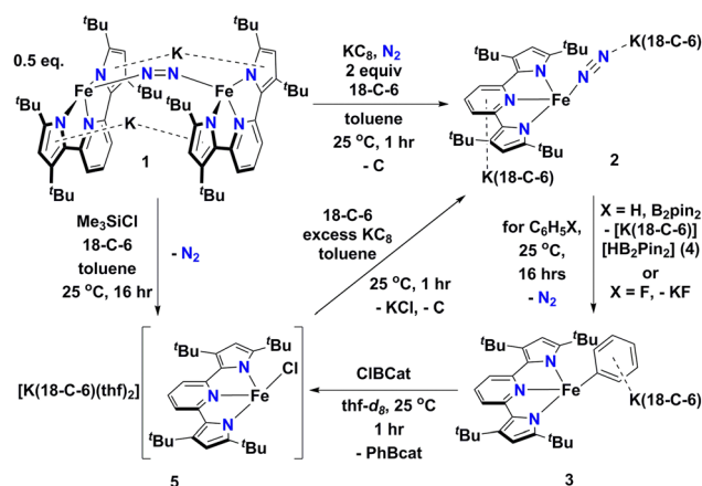
Scheme 1 Reaction scheme outlining formation and reactions of \{[K(18\text{-C-6})]_2(t^{\text{Bu}}\text{pyrr}_2\text{pyr})\text{Fe}(\text{N}_2)\} (2).
