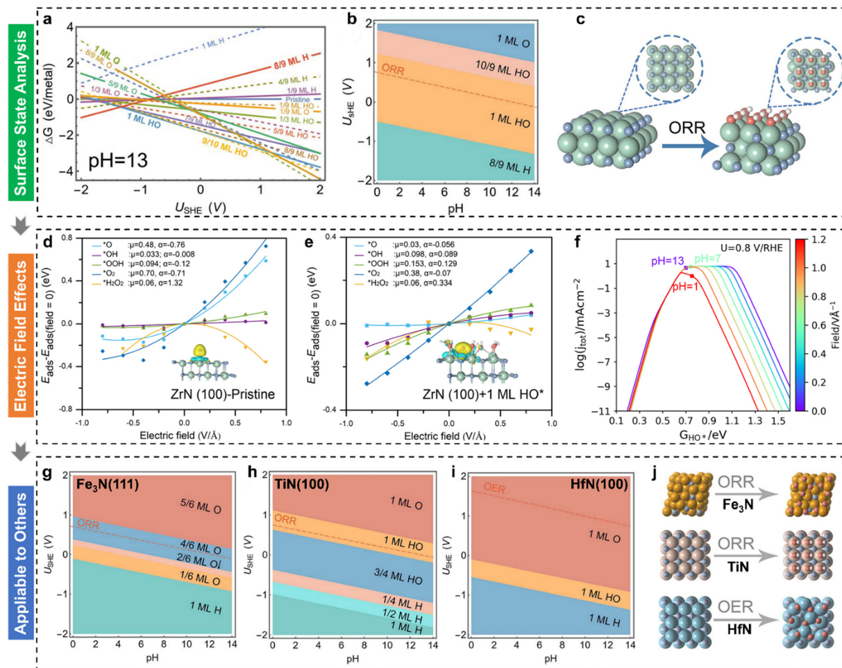
Fig. 3 (a) Calculated 1D surface Pourbaix diagram as a function of applied potential ( U_{\text{SHE}} ) ( T = 298.15 K, \text{pH} = 13 ); (b) calculated 2D surface Pourbaix diagram as a function of U_{\text{SHE}} and \text{pH} ( T = 298.15 K); (c) optimized ZrN(100) surface structures before and after the coverage of ^*\text{OH} under the ORR; electric field effects on ORR intermediates with fitted parameters for (d) pristine and (e) 1 \text{ ML HO}^* -covered ZrN(100); (f) derived pH-dependent volcano activity model for the ORR as a function of \text{HO}^* adsorption; calculated 2D surface Pourbaix diagrams as a function of U_{\text{SHE}} and \text{pH} ( T = 298.15 K) for (g) \text{Fe}_3\text{N}(111) , (h) \text{TiN}(100) , and (i) \text{HfN}(100) , respectively; (j) corresponding atomic structure evolutions under ORR conditions. 56
