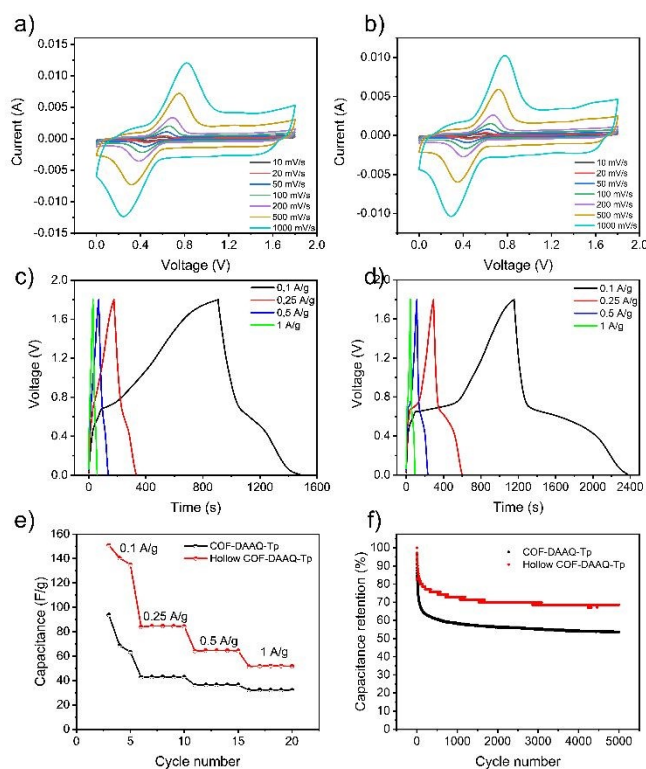
Fig. 3. Electrochemical characterization of COF-DAAQ-Tp and hollow COF-DAAQ-Tp. a-b) CV curves at different scan rates (0.01 – 1 V/s), and c-d) GCD at different current densities (0.1 – 1 A/g) for a, c) COF-DAAQ-Tp and b, d) hollow COF-DAAQ-Tp, e) rate performance COF-DAAQ-Tp (black curve) and hollow COF-DAAQ-Tp (red curve) at different current densities (0.1 – 1 A/g), and f) cycling performance at current density 1 A/g for 5000 charge/discharge cycles of COF-DAAQ-Tp (black curve) and hollow COF-DAAQ-Tp (red curve).
