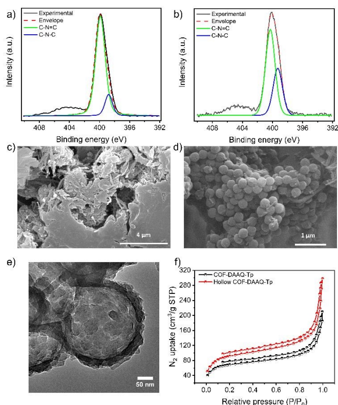
Fig. 2. a–b) N1s XPS analysis of a) COF-DAAQ-Tp, and b) hollow COF-DAAQ-Tp, c–d) SEM images of c) PS@COF-DAAQ-Tp and d) COF-DAAQ-Tp, e) HRTEM image of hollow COF-DAAQ-Tp and f) BET surface area of COF-DAAQ-Tp (black curve) and hollow COF-DAAQ-Tp (red curve).
