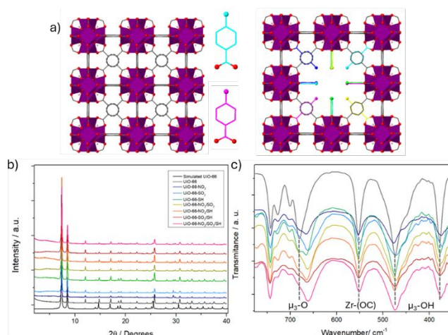
Fig. 1: a) Schematic representation of MTVM MOF with defect-induced re o topology in comparison with the pristine MOF. b) PXRD profiles c) amplification of FT-IR profiles highlighting μ 3 -O, μ 3 -OH and Zr-(OC) bands.
