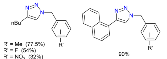
Scheme 39 Substrate scope of CuAAC reaction.
