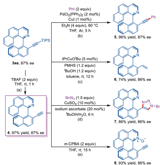
Scheme 3 Representative derivatizations.
