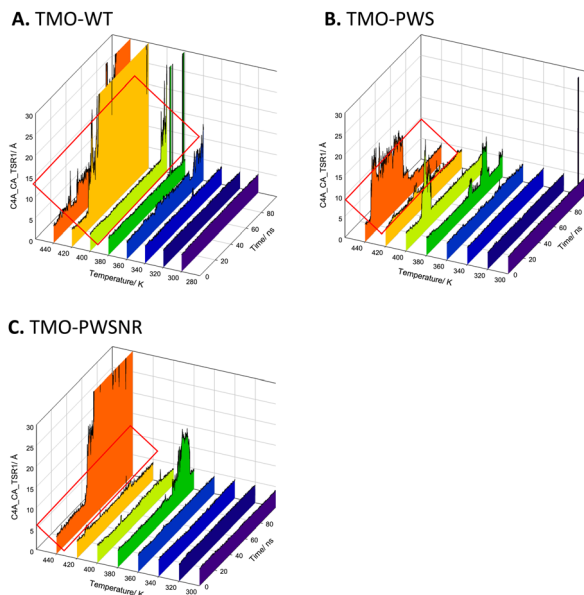
Fig. 9 Distances between the FAD cofactor and IAM (product) ( C_{4A}FAD-C_A TSR ) at different temperatures (300–440 K) of TMO-WT, TMO-PWS, and TMO-PWSNR variants. C_{4A}FAD-C_A TSR distance during 100 ns MD simulations for (A) TMO-WT, (B) TMO-PWS, and (C) TMO-PWSNR variants at 300–440 K. The red rectangle indicates large fluctuations of the residue pair.
