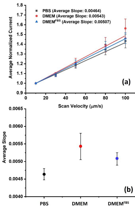
Fig. 4 Effect of different media on the electrochemical current response of HeLa cells. (a) Linear dependency of the average normalized peak current with respect to the scan velocity in PBS (black), DMEM (red), and DMEM FBS (blue). (b) Comparison of average slope in different media indicating higher electrochemical cell response in DMEM.
