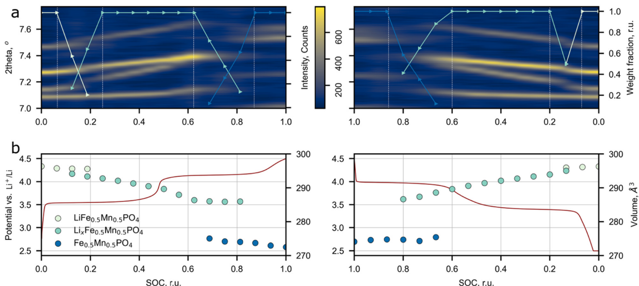
Fig. 6 Synchronized results of operando SXR study of Li-rich LFMP. (a) Evolution of peak positions and phase weights during cycling. (b) The unit cell volume change during cycling and charge–discharge profile at C/5.
