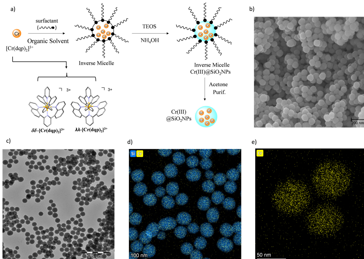
Fig. 3 (a) Schematic synthetic approach for preparing the silica nanoparticles (b) SEM image of the prepared rac -Cr@SiO 2 NPs (c) TEM image of the prepared \lambda\lambda -Cr@SiO 2 NPs; (d) and (e) HAADF-STEM compositional mapping image of \lambda\lambda -Cr@SiO 2 NPs.
