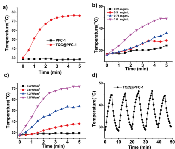
Fig. 2 Photothermal study of aqueous TQC@PFC-1 solution. (a) Comparison of the photothermal effect of PFC-1 and TQC@PFC-1 dispersed in aqueous solution ( 1 \text{ mg mL}^{-1} ) under 1080 \text{ nm} laser irradiation ( 1.5 \text{ W cm}^{-2} ). (b) Photothermal conversion of TQC@PFC-1 with different concentrations ( 0.25\text{--}1 \text{ mg mL}^{-1} ) under 1080 \text{ nm} laser irradiation ( 0.8 \text{ W cm}^{-2} ). (c) Photothermal conversion of TQC@PFC-1 aqueous solution ( 1 \text{ mg mL}^{-1} ) under 1080 \text{ nm} laser irradiation with different exposure intensities ( 0.4\text{--}1.5 \text{ W cm}^{-2} ). (d) Photothermal stability study of TQC@PFC-1 in aqueous solution ( 1 \text{ mg mL}^{-1} , 1080 \text{ nm} , 0.8 \text{ W cm}^{-2} ) during five cycles of heating-cooling processes.
