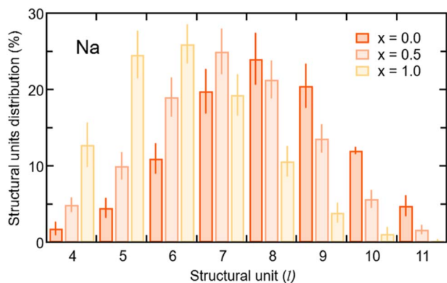
Fig. 6 Distributions of the structural units for Na of amorphous Na 3-x OH x Cl ( x = 0, x = 0.5 , and x = 1 ) as a function of the number of neighbors in each unit ( l ). Values obtained by using the definition of "total" coordination n_{ij}^t , given in Section 3.1.3.
