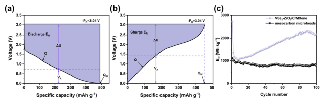
Fig. 5 Typical legends for the determination of the relative energy density ( E_R ) of (a) discharge E_R and (b) charge E_R . (c) Discharge E_R of VSe_2-ZrO_2/C/MXene and meso-carbon microbeads.
