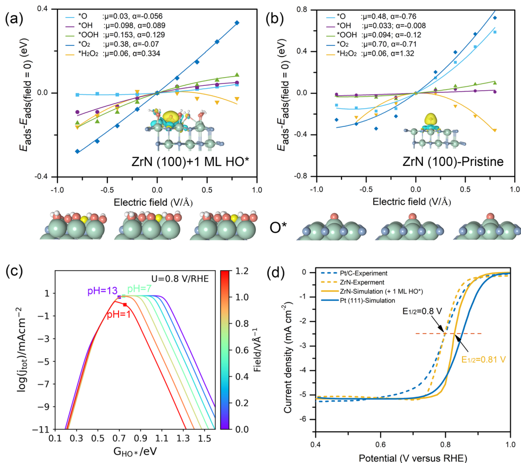
Fig. 4 Electric field effects and pH-dependent microkinetic modelling. (a) Electric field effects on ORR adsorbates with fitted values for \mu (e) and \alpha ( \text{e}^2 \text{V}^{-1} ) for 1 ML \text{HO}^* -covered ZrN(100) and (b) pristine ZrN(100). Insets show the calculated charge density difference induced by \text{O}^* adsorption, where yellow and cyan represent charge accumulation and loss, respectively. (c) Derived pH-dependent volcano activity model for the ORR as a function of \text{HO}^* adsorption (at 0.8 \text{ V} vs. RHE). (d) Simulated ORR polarization curves on 1 ML \text{HO}^* -covered ZrN(100) and Pt(111), plotted along with the experimental polarization curves for ZrN and Pt/C. 21 Insets are the optimized structures with \text{O}^* adsorption under different electric fields ( -0.6, 0 , and 0.6 \text{ V}/\text{\AA} ). Green, blue, red, and white spheres represent Zr, N, O, and H, respectively. The adsorbed O for structures in (a) is marked in yellow.
