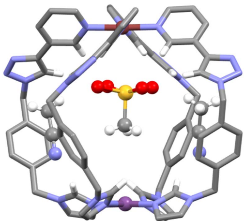
Fig. 5 Molecular structure of the C \subset Mso^- host–guest adduct. The Mso^- guest is rotationally disordered. Colours: Pd II brick, Pt II purple, N periwinkle blue, C grey, H white, O red, S orange. Hydrogen atoms involved in H-bonding interactions are shown. All other hydrogen atoms, most solvents of crystallisation and counterions have been omitted for clarity.
