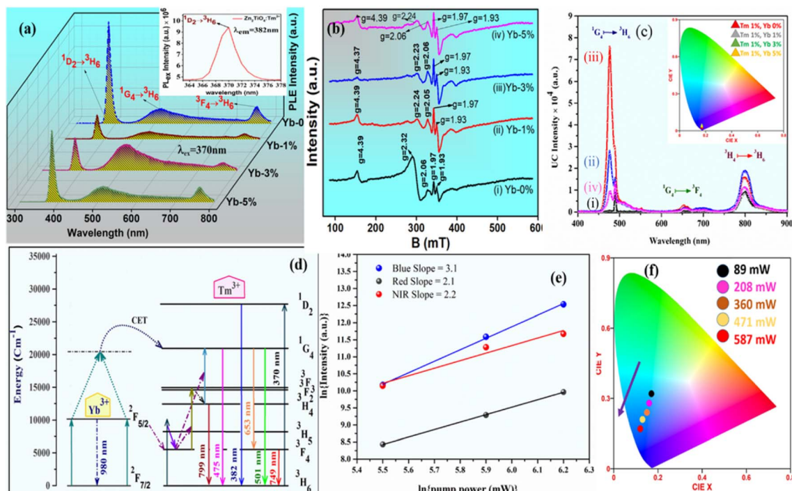
Fig. 5 (a) PL emission spectra at 370 nm excitation wavelength. The inset represents the excitation spectrum of \text{Zn}_2\text{TiO}_4:\text{TM}^{3+} phosphor at 382 nm emission. (b) and (c) represents the EPR intensity and UC emission spectra of the powder samples (i) \text{Zn}_2\text{TiO}_4:\text{TM}^{3+}\text{-1\%, Yb}^{3+}\text{-0\%} (ii) \text{Zn}_2\text{TiO}_4:\text{TM}^{3+}\text{-1\%, Yb}^{3+}\text{-1\%} (iii) \text{Zn}_2\text{TiO}_4:\text{TM}^{3+}\text{-1\%, Yb}^{3+}\text{-3\%} (iv) \text{Zn}_2\text{TiO}_4:\text{TM}^{3+}\text{-1\%, Yb}^{3+}\text{-5\%} respectively recorded at room temperature. The inset of (c) shows the CIE plot of UC emission intensity. (d) Schematic energy level diagram (e) pump power dependence study of \text{TM}^{3+}\text{-Yb}^{3+} codoped \text{Zn}_2\text{TiO}_4 phosphors (f) The corresponding CIE plot of the pump power variation in the optimized sample.
