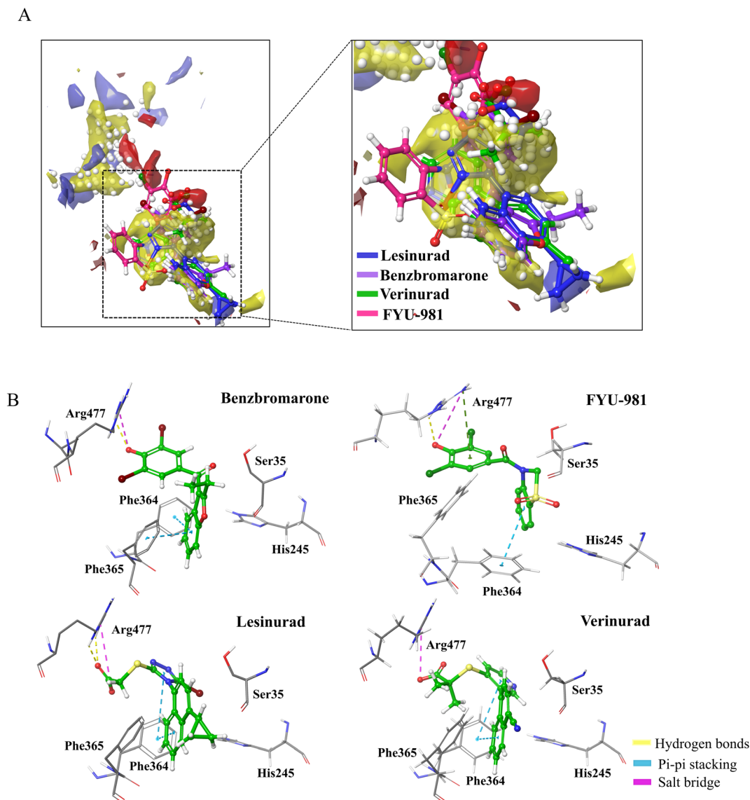
Fig. 2 SiteMap predict binding pocket and docking results. (A) The pocket predicted by SiteMap (left) can be superimposed with the four positive structures docked using IFD (right). (B) The 3D interaction pattern diagram of URAT1 and four known drugs using IFD.
