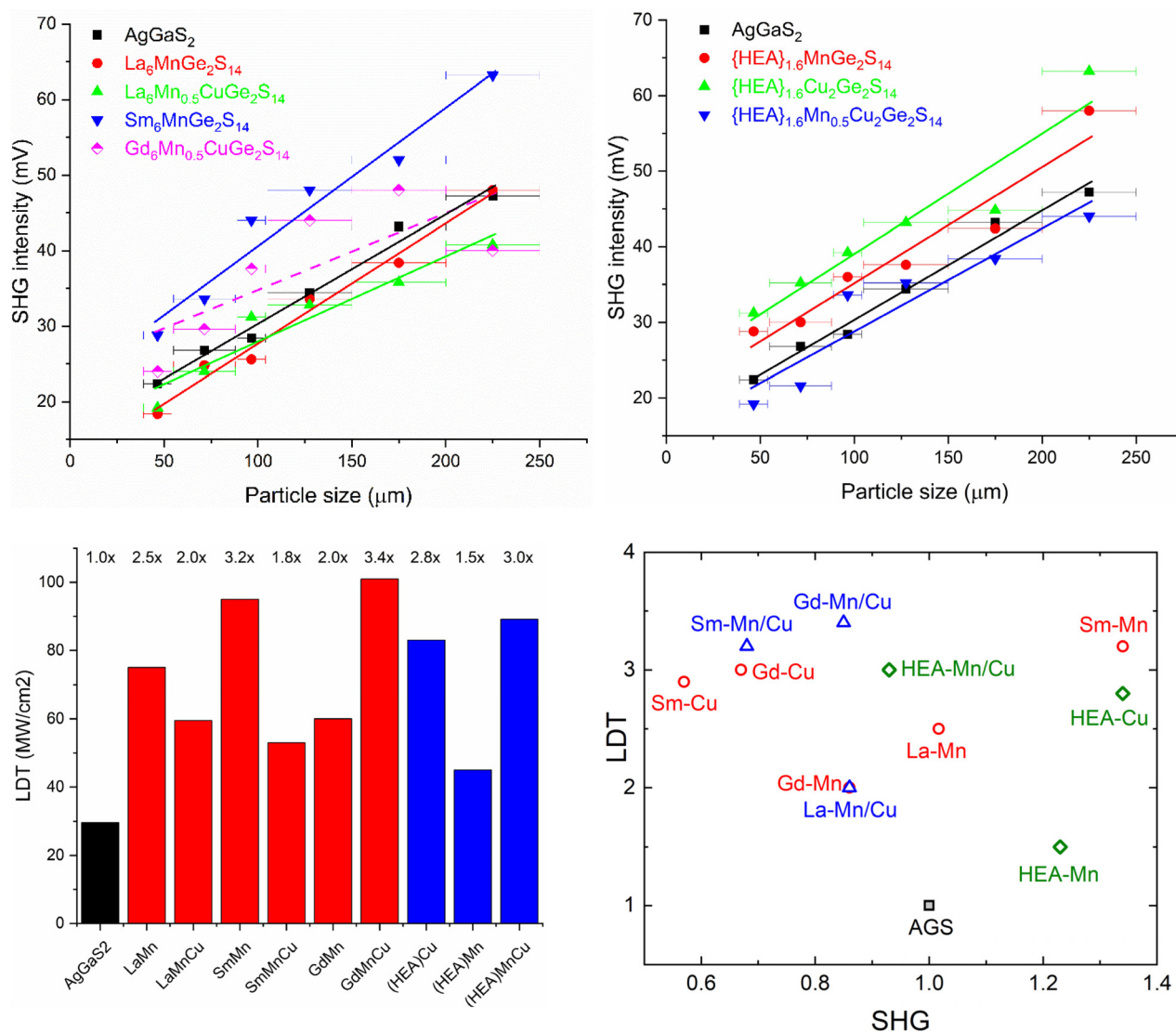
Fig. 4 (Top) Second-harmonic generation (SHG) intensity for (A)_6(TM)Ge_2S_{14} compositions ( A = La, Sm, Gd , HEA = YLaCeSmGd, TM = Mn, Cu ). The solid lines are drawn to guide the eye. All compositions are phase matchable except Gd_6Mn_{0.5}CuGe_2S_{14} (shown with a dashed pink line). (Bottom Left) Laser damage threshold (LDT) intensities for (A)_6(TM)Ge_2S_{14} compositions. Numbers above the columns indicate the value of LDT relative to the standard AgGaS_2 . Standard AgGaS_2 is shown in black in all panels. (Bottom right) SHG/LDT diagram showing SHG values at the maximum studied particle size and LDT values normalized to those for the AGS standard. Data for single RE–Cu compositions are taken from ref. 24.
