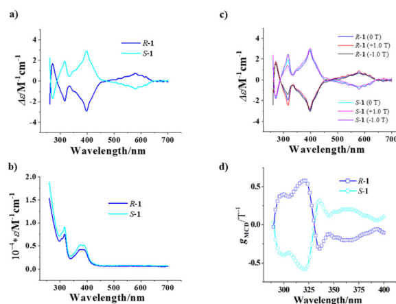
Fig. 5 CD spectra of R -1 and S -1 at room temperature (MeCN, c = 0.2 g L −1 , optical path = 1 mm) (a). UV-visible spectra of R -1 and S -1 at room temperature (MeCN, c = 0.2 g L −1 , optical path = 1 mm) (b). CD spectra in a MeCN solution at room temperature ( c = 0.2 g L −1 , optical path = 1 mm, H = 0 and \pm 1.0 T) (c). g_{MCD} of R -1 and S -1 (d).
