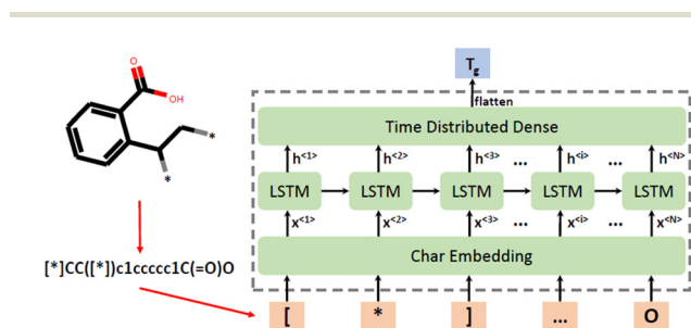
Fig. 6 Polymer representation processing and ML model structure. Reproduced from ref. 51 with permission from MDPI, copyright 2021.
