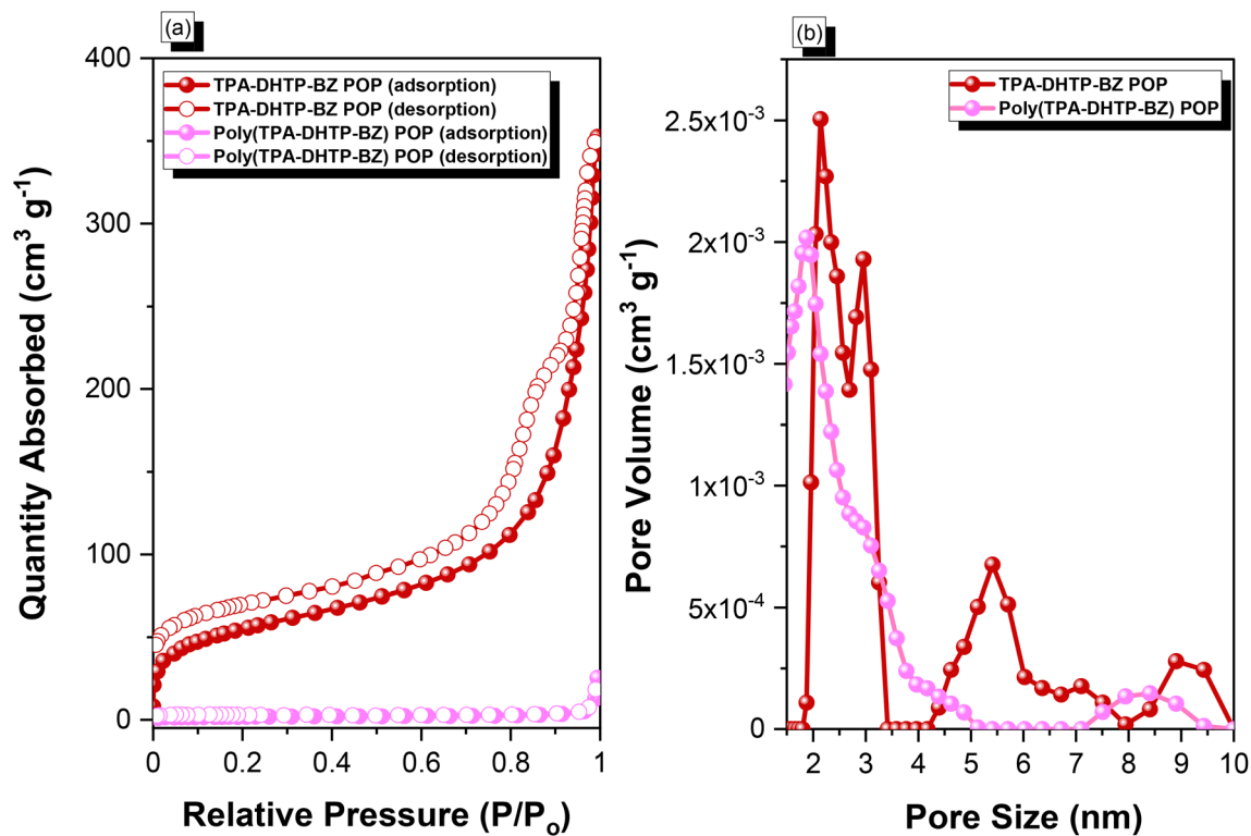
Fig. 7 (a) \text{N}_2 adsorption/desorption isotherms at 77 K and (b) pore size distributions of the TPA-DHTP-BZ POP and poly(TPA-DHTP-BZ) POP.
