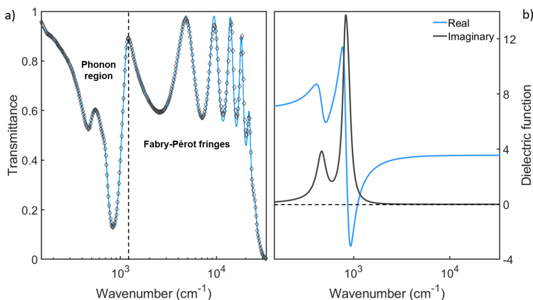
Fig. 1 (a) Experimental (light blue line) and fitted (black empty diamond symbols) transmittance of the Si 3 N 4 membrane, measured in the THz-UV range. The vertical black dashed line separates the phonon absorption region (low-frequency) to the high-frequency part characterized by Fabry-Pérot fringes. (b) Real (light blue line) and imaginary (black line) parts of the dielectric function, extracted from the fitted transmittance by considering the Fabry-Pérot effect.
