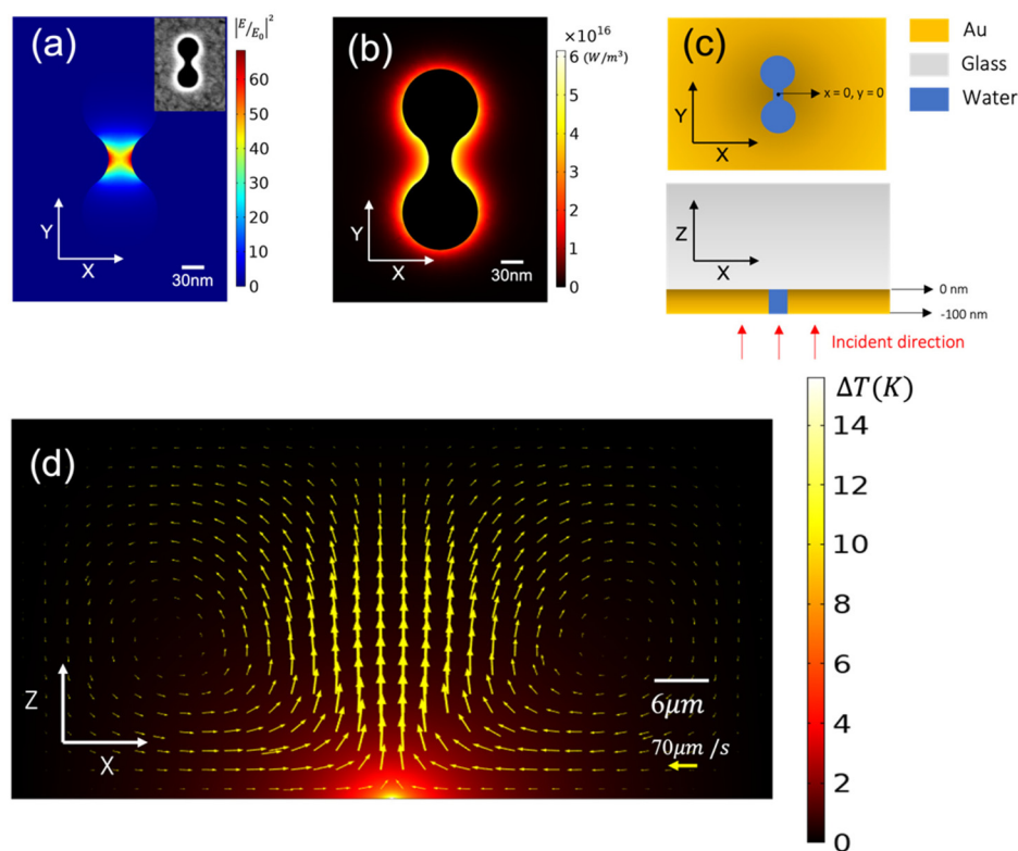
Fig. 2 Optical and thermal simulations. (a) FEM simulation showing the intensity enhancement in the XY plane at Z = -20 \text{ nm} . This shows intense enhancement in the gap of the DNH. The inset shows an SEM micrograph of the DNH aperture. (b) Optical power dissipation density in the XY plane at Z = -50 \text{ nm} , showing that the optical power dissipated in the Au film by the plasmonic aperture is very tightly confined to the vicinity of the DNH. (c) Schematic design of the DNH aperture showing how the axes are defined. (d) ZX cross section at Y = 0 showing the distribution of the temperature rise and the velocity vector plot, with the vector arrows proportional to the magnitude of the velocity vector resulting from a Gaussian beam with an intensity of 11.4 \text{ mW } \mu\text{m}^{-2} and beam diameter 1.33 \text{ } \mu\text{m} . This shows a maximum temperature rise of 15 \text{ K} and velocity magnitudes exceeding 70 \text{ } \mu\text{m s}^{-1} for a 10 \text{ VAC} at 20 \text{ kHz} .
