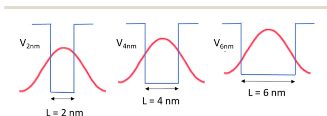
Fig. 7 Schematic of proposed mechanism of how wavefunction overlap in a PIB model differs with NP size in small ( L = 2 ), medium ( L = 4 ), and large ( L = 6 ) size regimes. The rectangles shown represent the comparative size of the boxes for each NP size. The red curve represents a simple n = 1 wavefunction for the NP exciton if it were not confined. V_{2 \text{ nm}} , V_{4 \text{ nm}} , and V_{6 \text{ nm}} represent the height of the boxes or the potential barriers, and are dependent on the ionization potentials of the respectively sized NPs.
