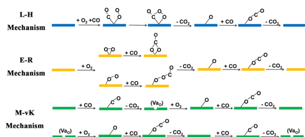
Scheme 1 Three different mechanisms of COOR catalysis.
