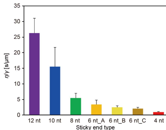
Fig. 2 Inverse capillary velocities of DNA droplets composed of Y-motifs with various SE designs at T_d (70, 61, 63, 48, 49, 43, and 46 °C for 12 nt, 10 nt, 8 nt, 6 nt A , 6 nt B , 6 nt C , and 4 nt). Error bars indicate standard deviations ( n = 12, 13, 13, 12, 19, 14, and 14 for SE designs of 12 nt, 10 nt, 8 nt, 6 nt A , 6 nt B , 6 nt C , and 4 nt, respectively).
