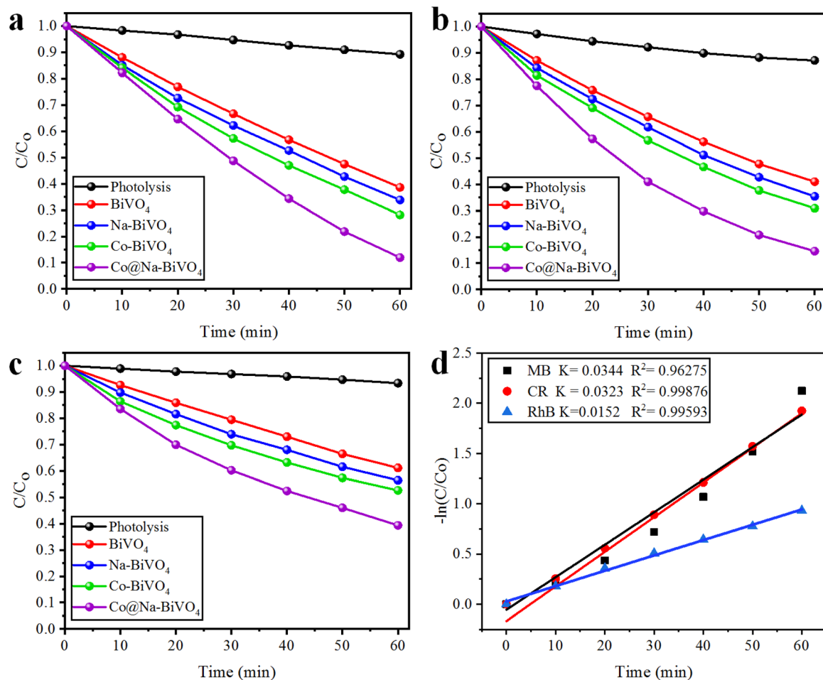
Fig. 7 Comparative degradation activities of dyes with photolysis (degradation via photons), \text{BiVO}_4 , Na- \text{BiVO}_4 , Co- \text{BiVO}_4 and Co@Na- \text{BiVO}_4 (a) MB, (b) CR and (c) RhB, whereas (d) represents the kinetic study for MB, CR and RhB obtained over Co@Na- \text{BiVO}_4 photocatalysts.
