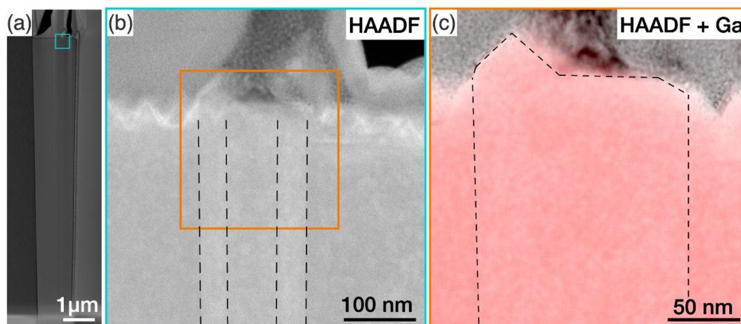
Fig. 5 (a) HAADF TEM images of a tall GaN nanowire with a protuberance structure on the top surface. (b) HAADF image of the area marked in (a) where the protuberance structure was expected. (c) EDX map of the Ga signal superimposed on the HAADF image of the area highlighted in (b) with the protuberance structure and the hexagonal prism highlighted by dashed lines.
